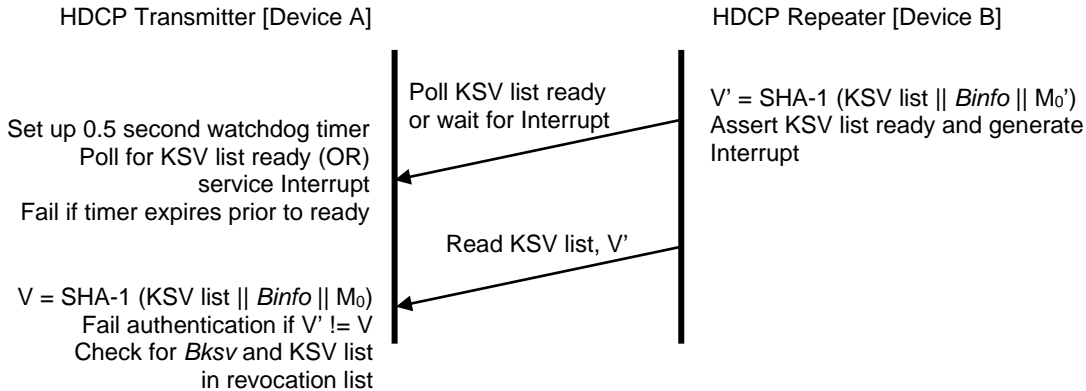
Figure 2-2. Second Part of Authentication Protocol
