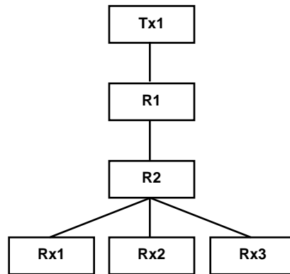
Figure 2-5. DEPTH and DEVICE_COUNT for HDCP Repeater
