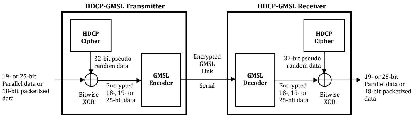
Figure 3-1. HDCP-GMSL Encryption and Decryption
