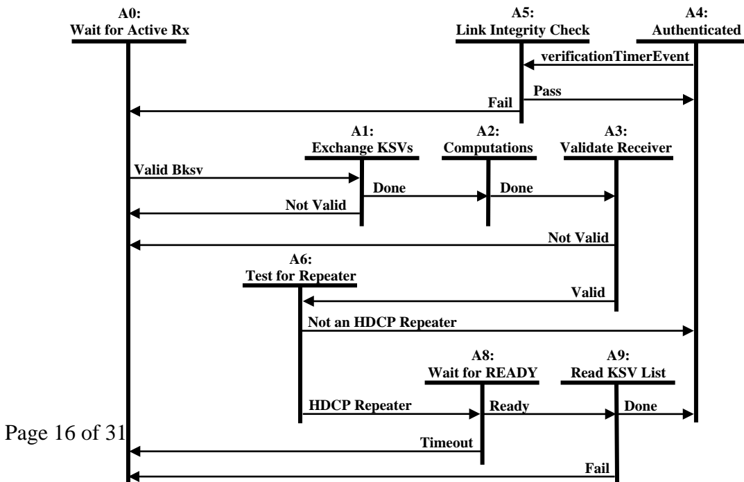
Figure 2-8. HDCP Transmitter Link State Diagram
